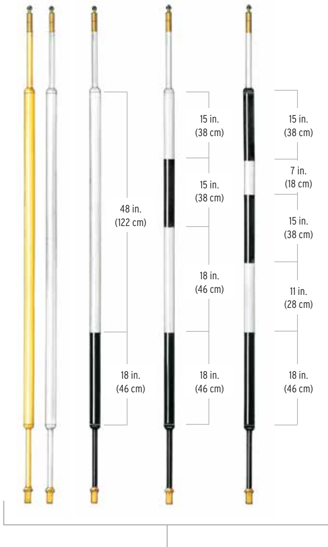
Aluminum/Fiberglass Tournament Flagsticks 1 in. (3 cm)
